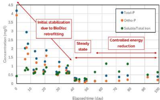
Figure 3: Phosphorus and Iron Concentrations at System Outlet
