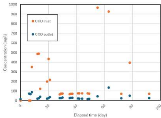
Figure 2: COD Concentrations at the Inlet and Outlet
